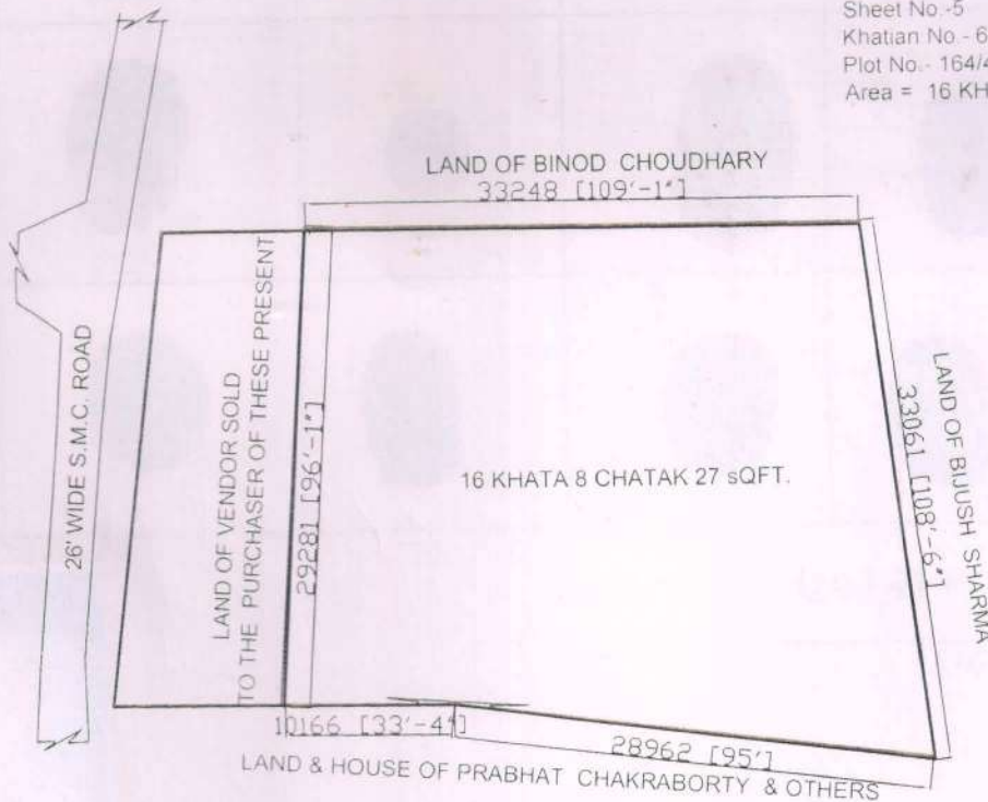
Site Plan Scale -1:500
